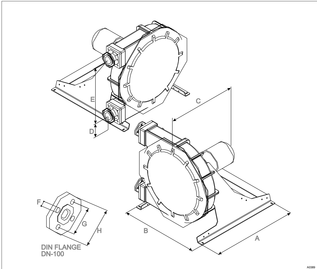
Fig. 22: Dimensions DFDa 100
